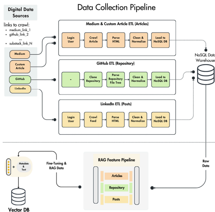
Figure 3.1: LLM Twin's data collection ETL pipeline architecture
